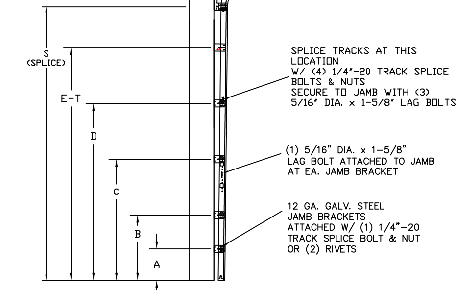
TRACK CONFIGURATION FOR UP TO 24' TALL DOORS N.T.S. SEE TABLE 2 FOR TRACK ATTACHMENT SPACING
